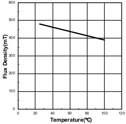
FLUX DENSITY(B) vs. TEMPERATURE
