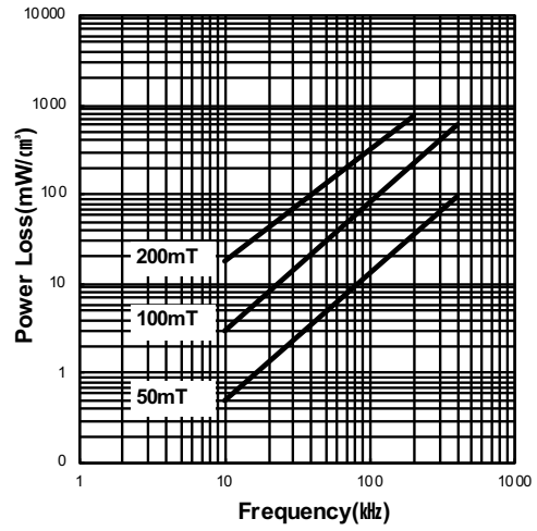
POWER LOSS( P_L ) vs. FREQUENCY at 25°C
