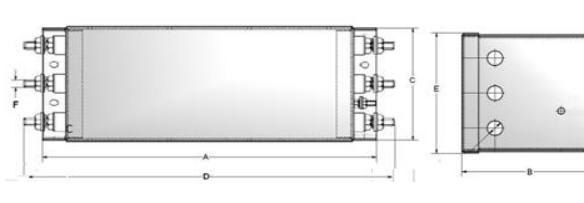
Fig 2 (Bolt type)
