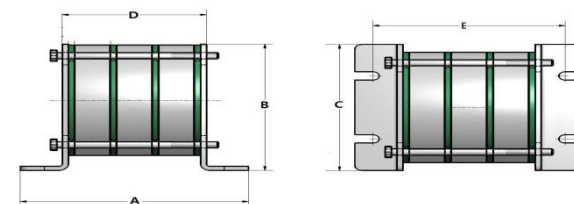
Fig 3 (FRAME TYPE)
